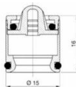
MSCLMT1015023 Flow regulator 10 lit/min
