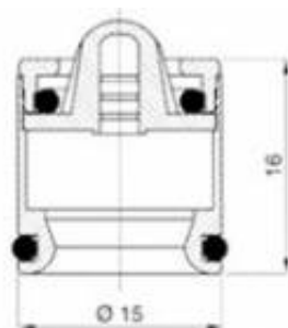
MSCLMT0815001 Flow regulator 8 lit/min
