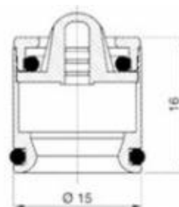
MSCLMT0615018 Flow regulator 6 lit/min
